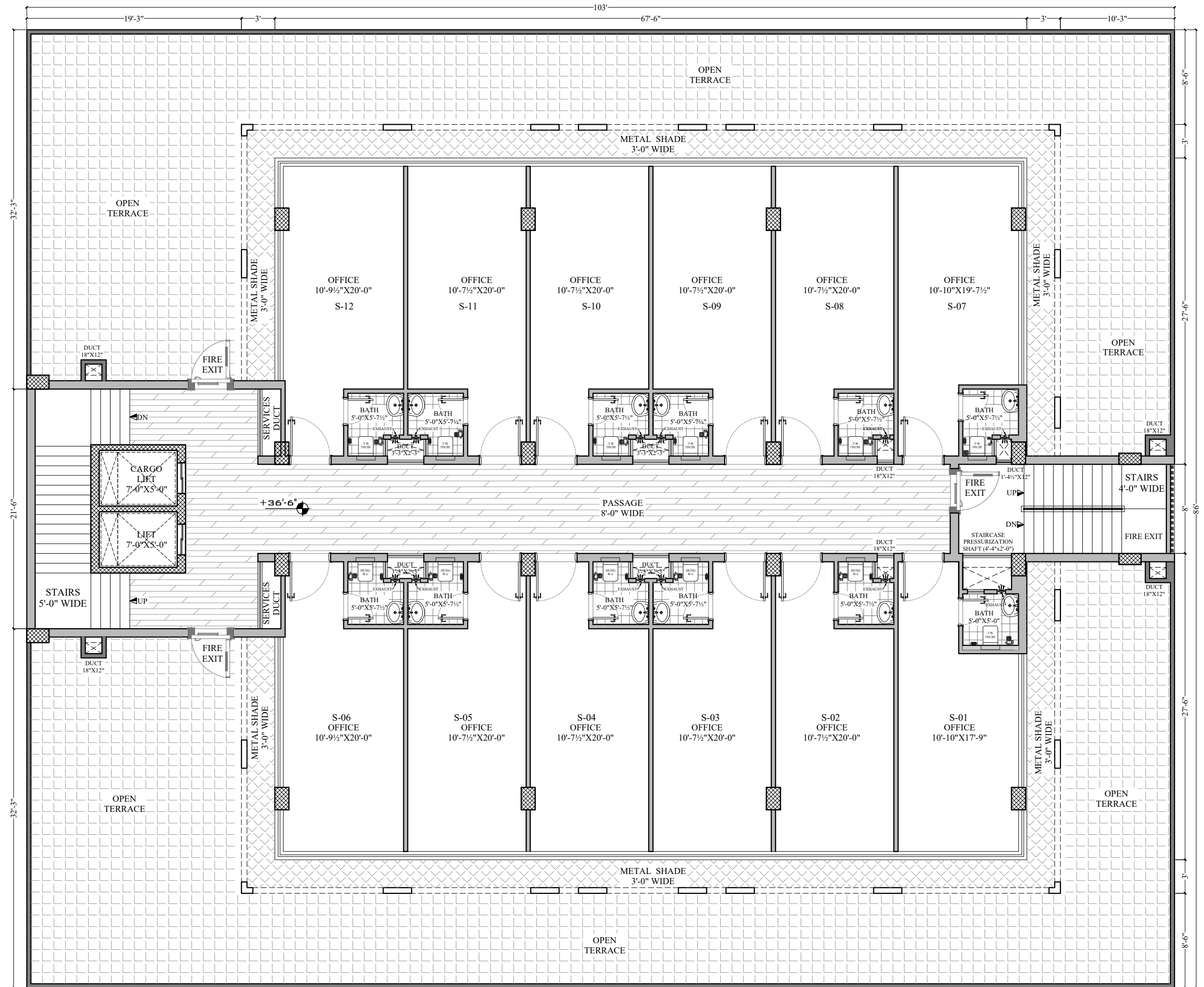
2nd and 3rd FLOOR PLAN
